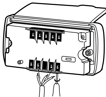
Connect the end of the cable into the control block.
