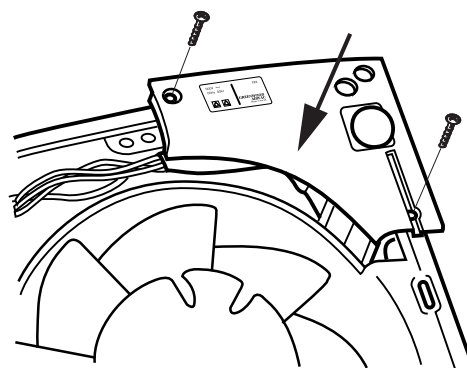
Screw the sensor module into position.
