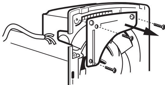
Release the electrical panel from the fan plate.
