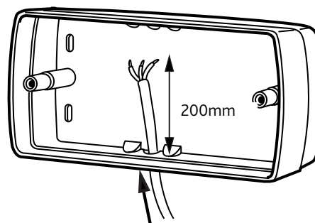
Feed approx. 200mm of supply cable into the box.
