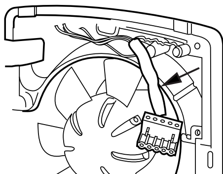
Lift out the sensor module wiring connector.
