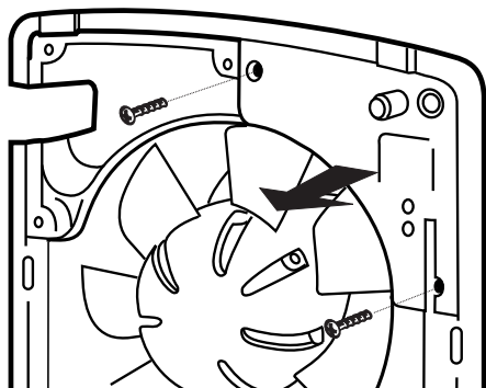
Unscrew the module plate from motor plate assembly.
