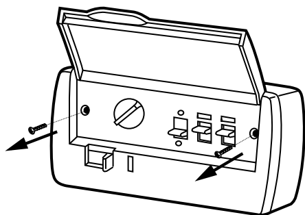
Lift up panel and remove two screws to dismantle unit.
