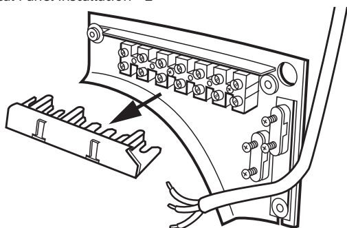
Remove the terminal cover.
