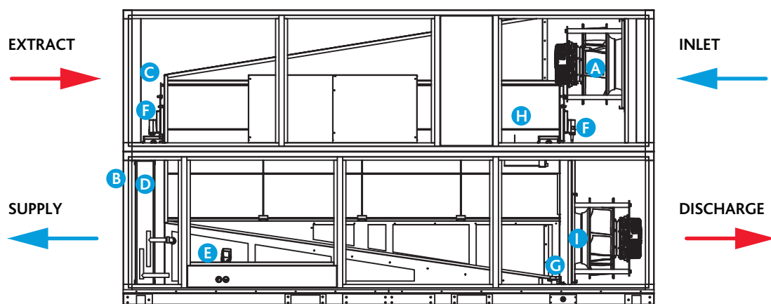
Figure 36b. XBC unit side view.
