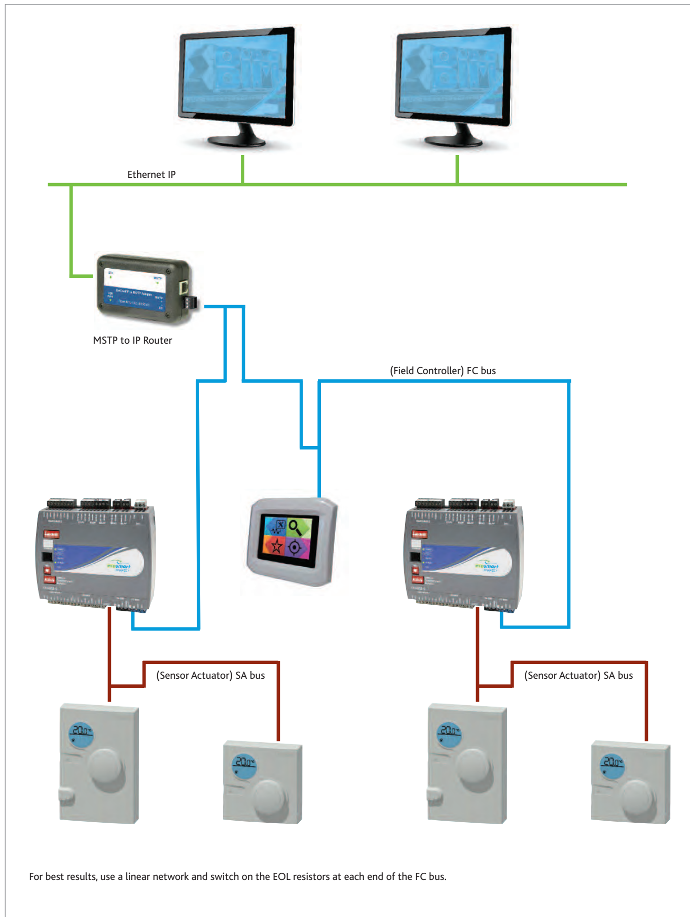
NETWORK CONNECTION DIAGRAM Figure 20:
