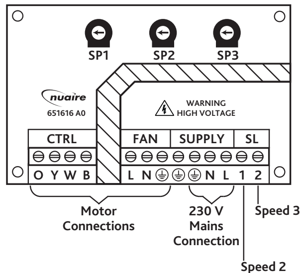
Figure 3. PCB
