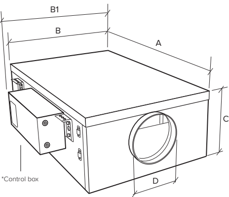
DIMENSIONS (mm) AND WEIGHT (Kg)
