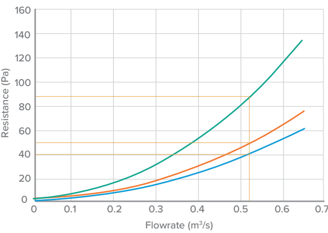
FILTER RESISTANCE - HIAQM-065
