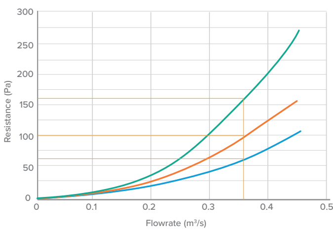
FILTER RESISTANCE - HIAQM-045
