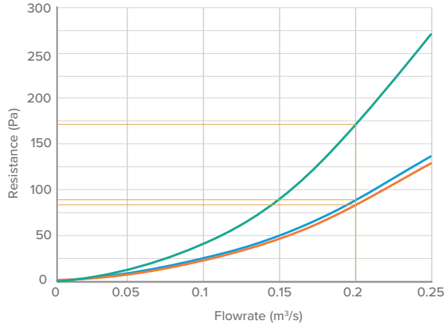
FILTER RESISTANCE - HIAQM-015
