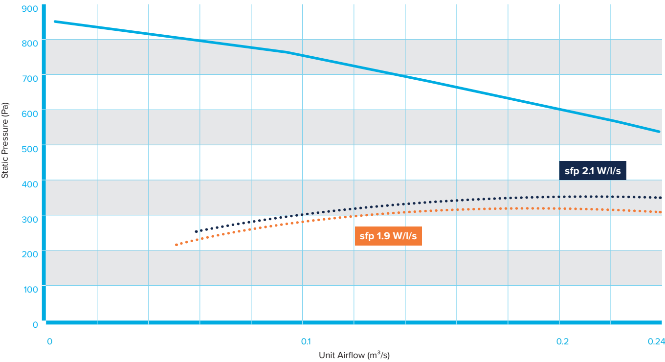
PERFORMANCE CHART
