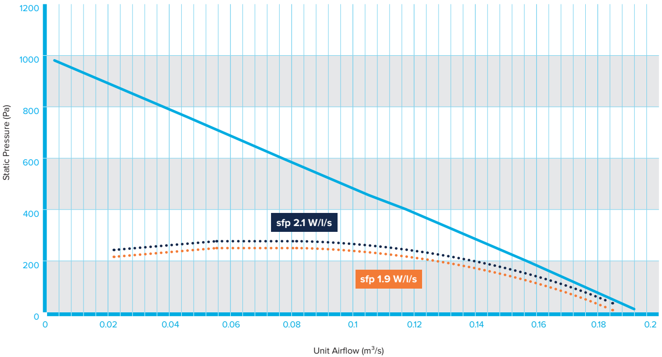
PERFORMANCE CHART
