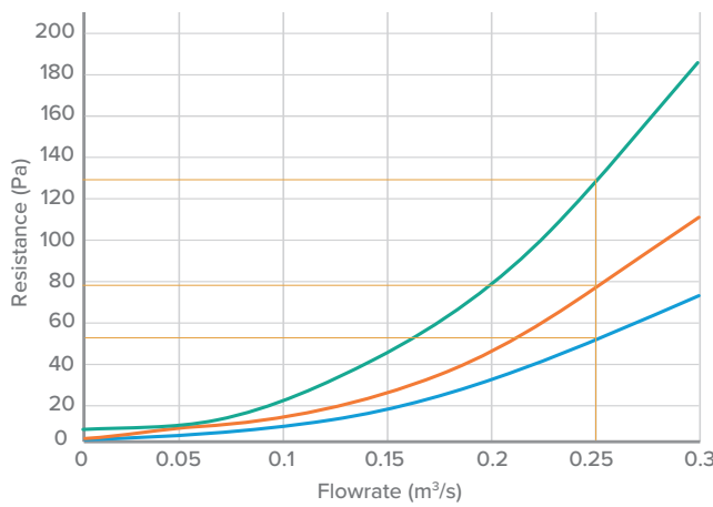
FILTER RESISTANCE - HIAQM-025
