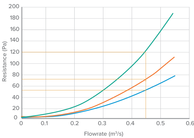
FILTER RESISTANCE - HIAQM-055
