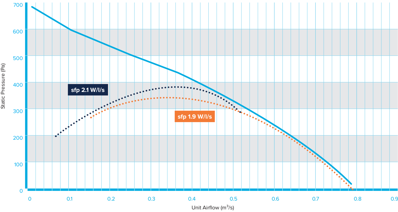
PERFORMANCE CHART
