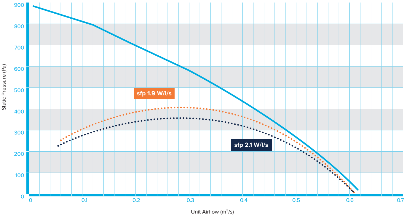
PERFORMANCE CHART
