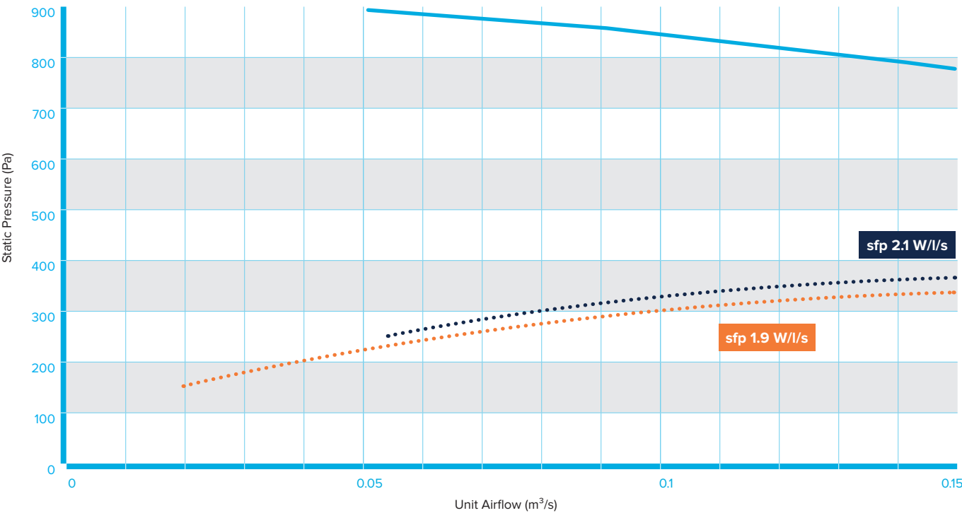
PERFORMANCE CHART
