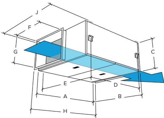
EXAMPLE UNIT: BOTTOM ACCESS INTERNAL UNIT
